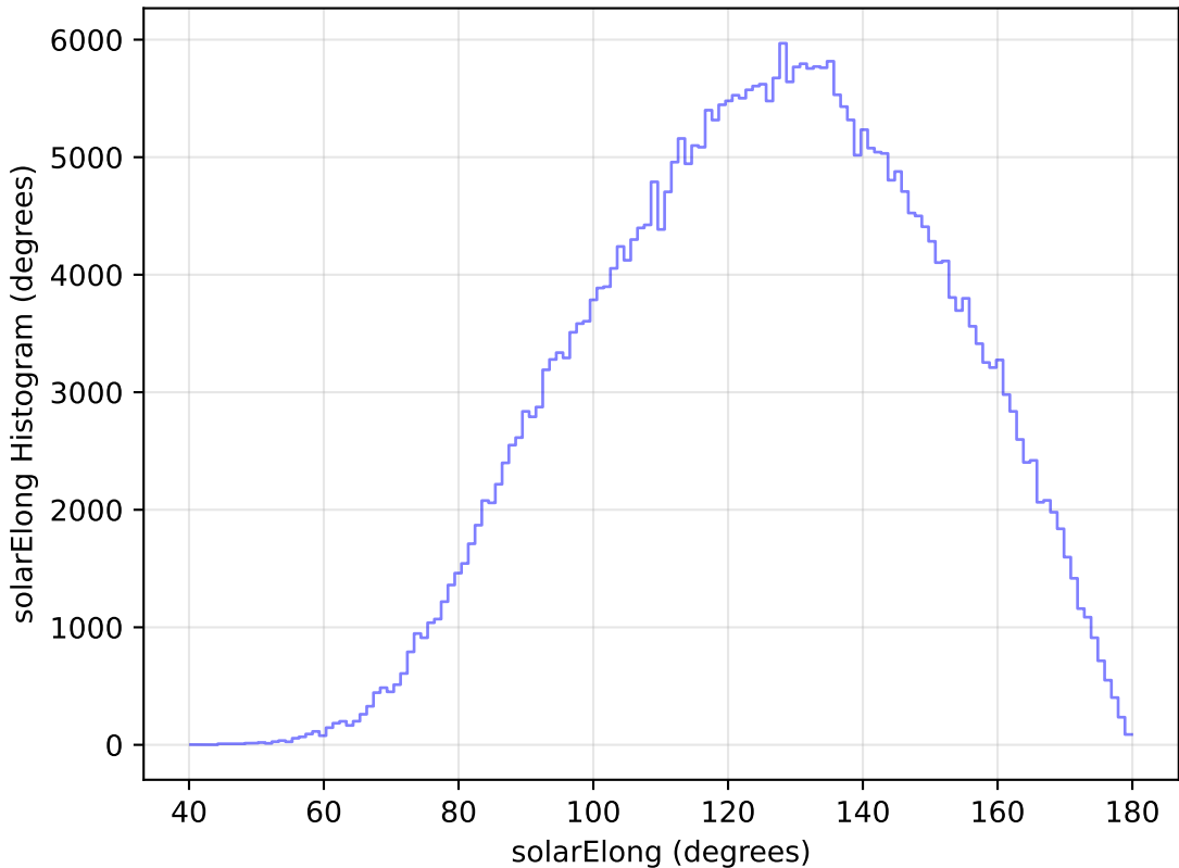
noroll_mjdp120_v3.4_10yrs All sky y band: solarElong Histogram
