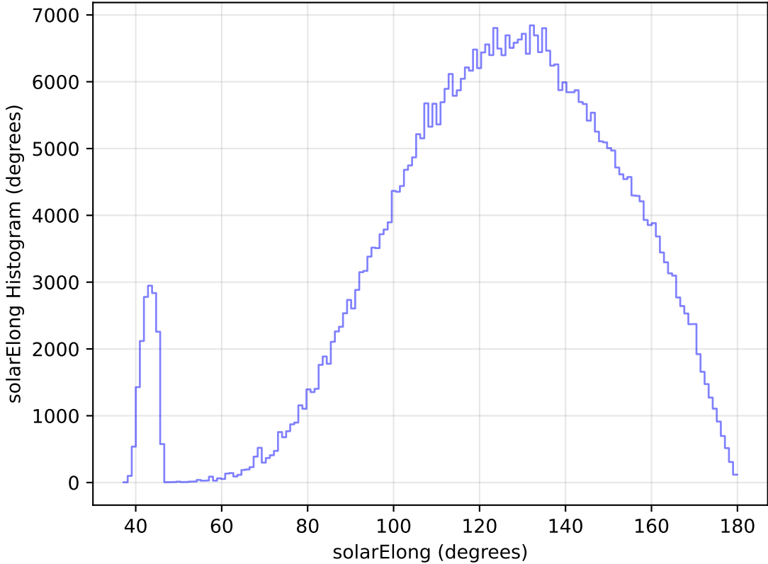
noroll_mjdp120_v3.4_10yrs All sky r band: solarElong Histogram
