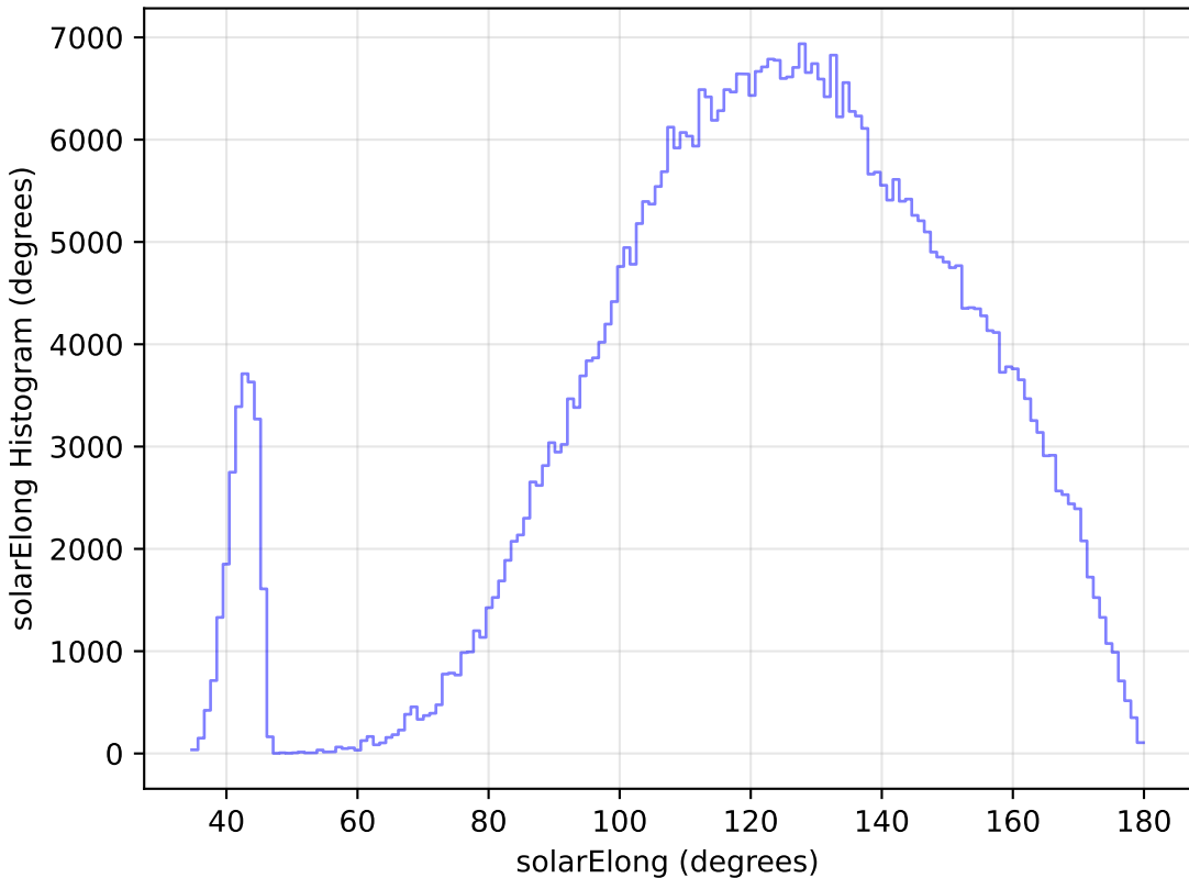
noroll_mjdp120_v3.4_10yrs All sky i band: solarElong Histogram
