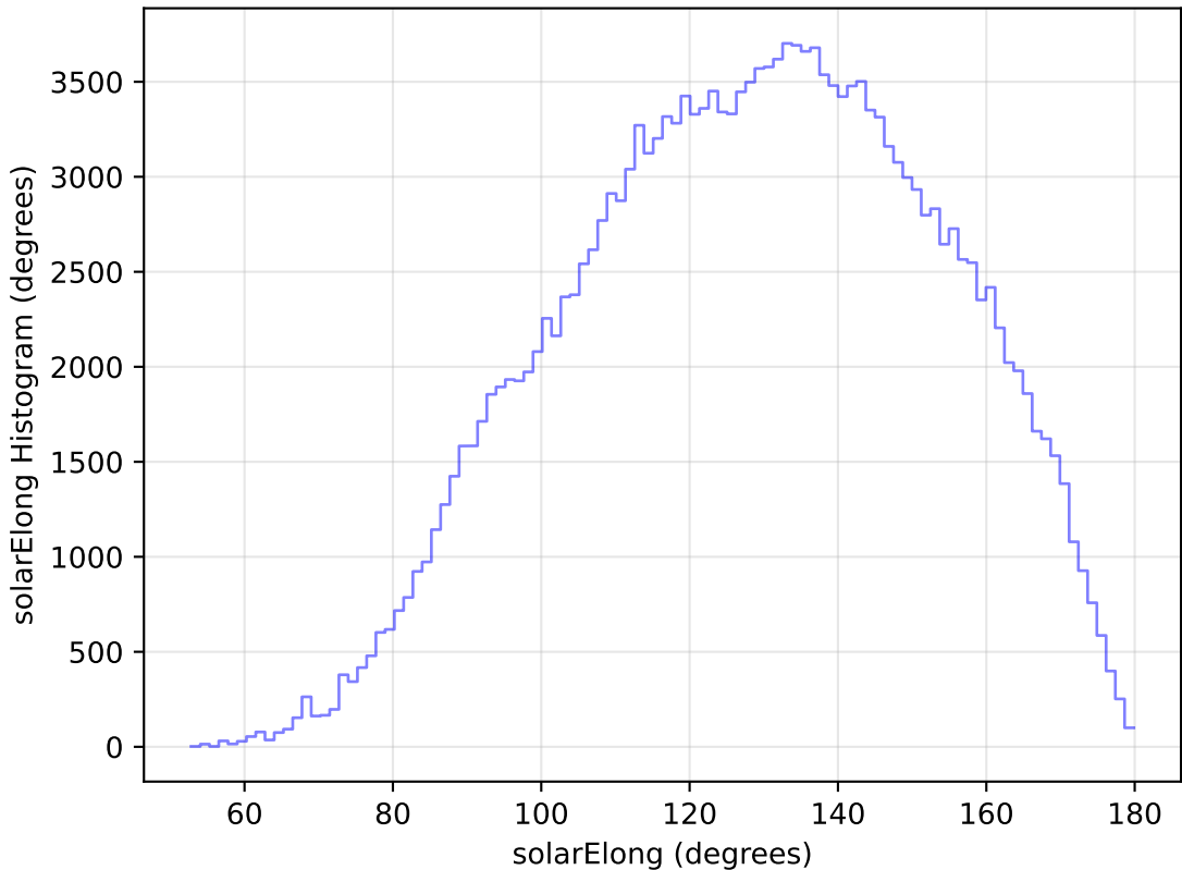
noroll_mjdp120_v3.4_10yrs All sky g band: solarElong Histogram
