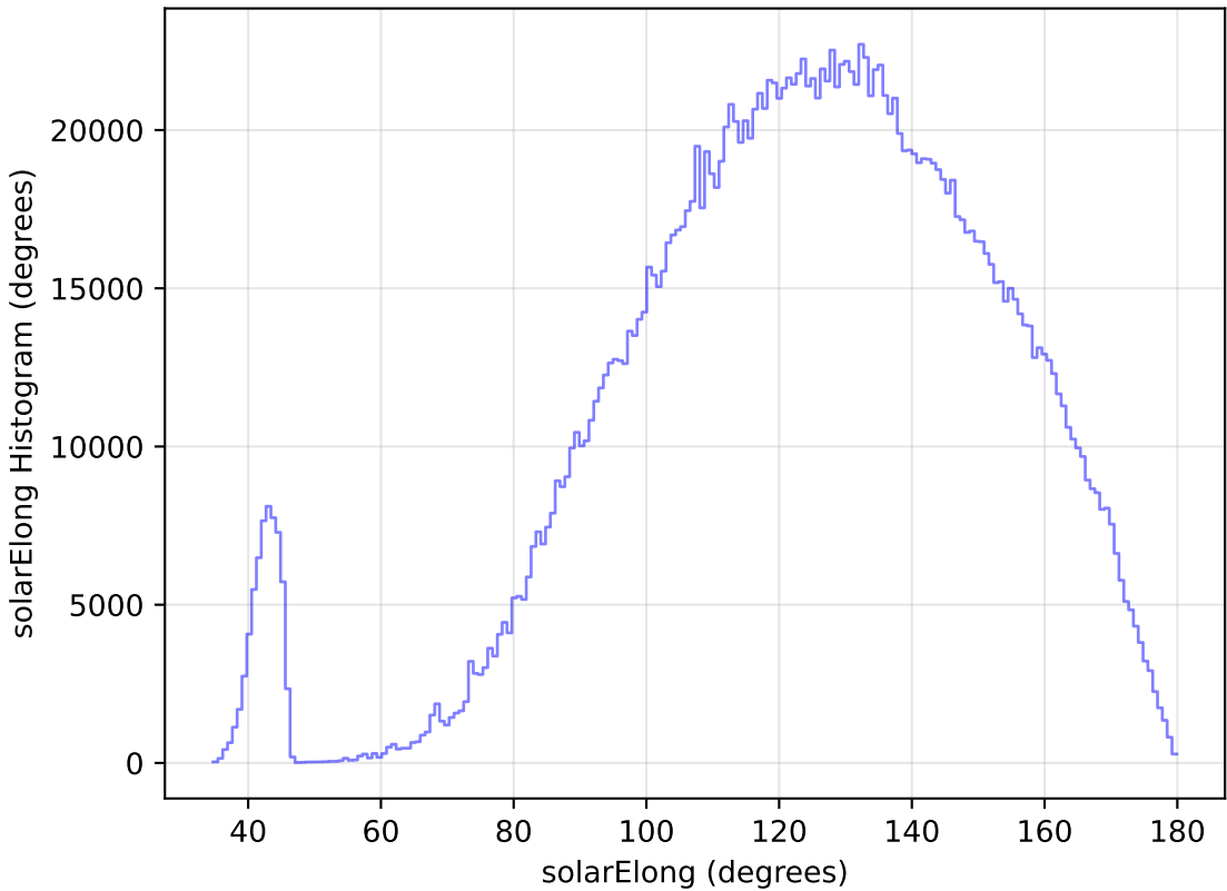
noroll_mjdp120_v3.4_10yrs All sky all bands: solarElong Histogram
