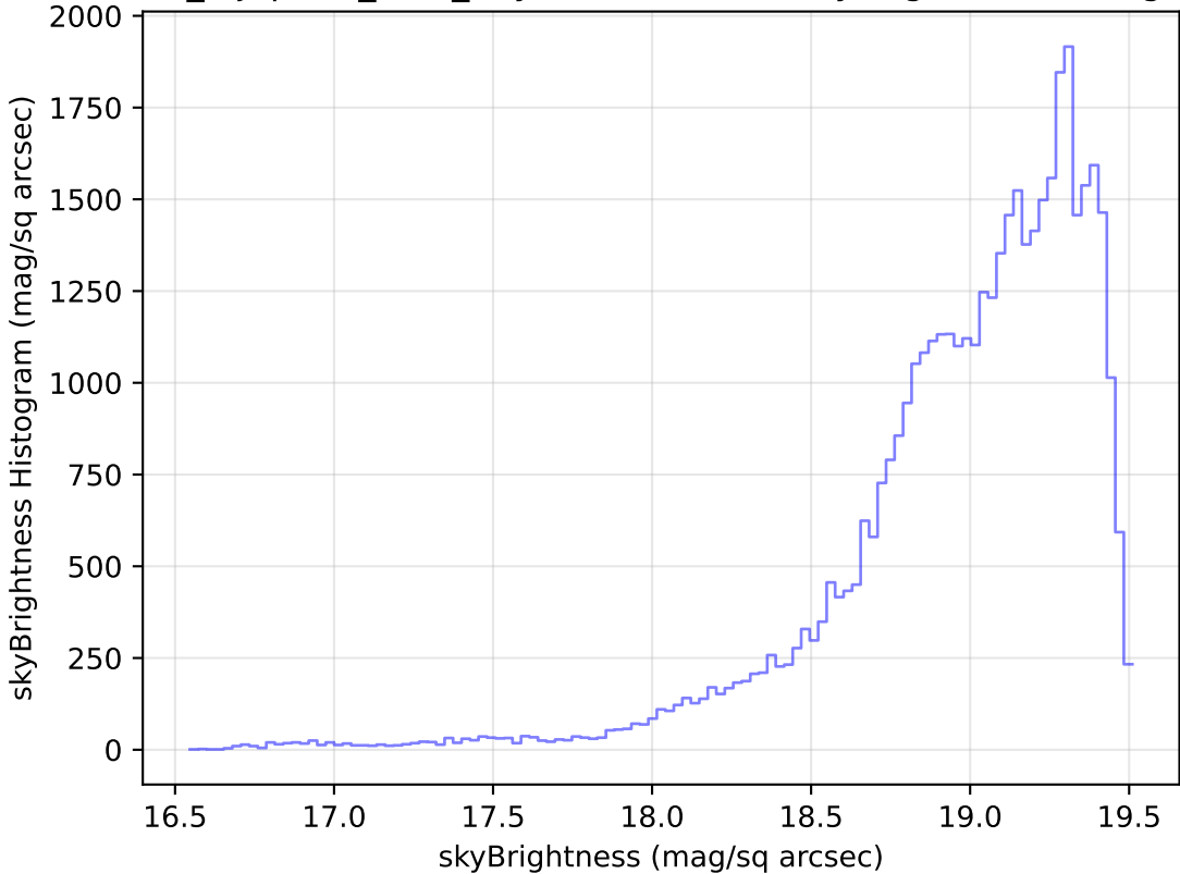
noroll_mjdp120_v3.4_10yrs Yr 1 z band: skyBrightness Histogram
