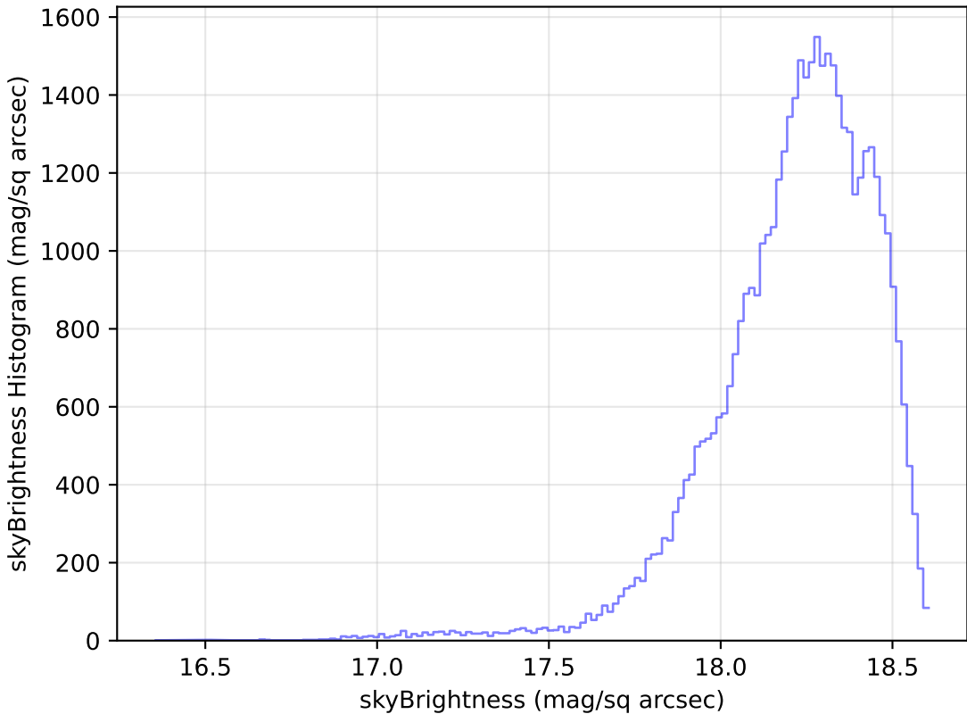
noroll_mjdp120_v3.4_10yrs Yr 1 y band: skyBrightness Histogram
