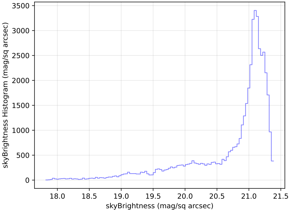
noroll_mjdp120_v3.4_10yrs Yr 1 r band: skyBrightness Histogram
