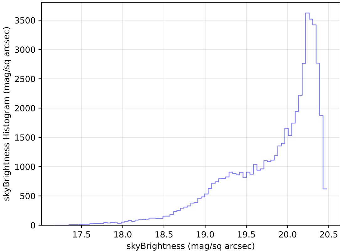
noroll_mjdp120_v3.4_10yrs Yr 1 i band: skyBrightness Histogram
