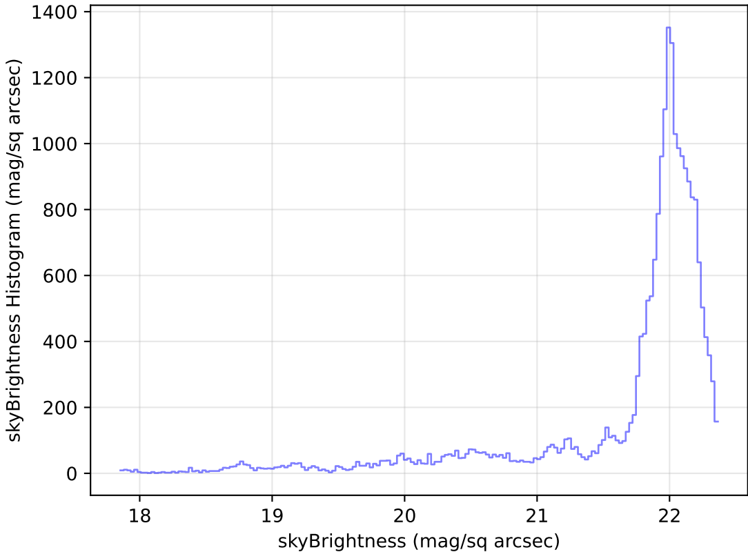
noroll_mjdp120_v3.4_10yrs Yr 1 g band: skyBrightness Histogram
