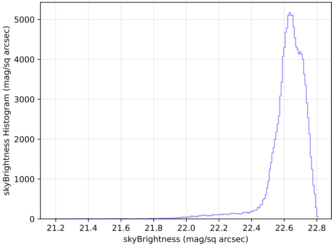
noroll_mjdp120_v3.4_10yrs WFD u band: skyBrightness Histogram
