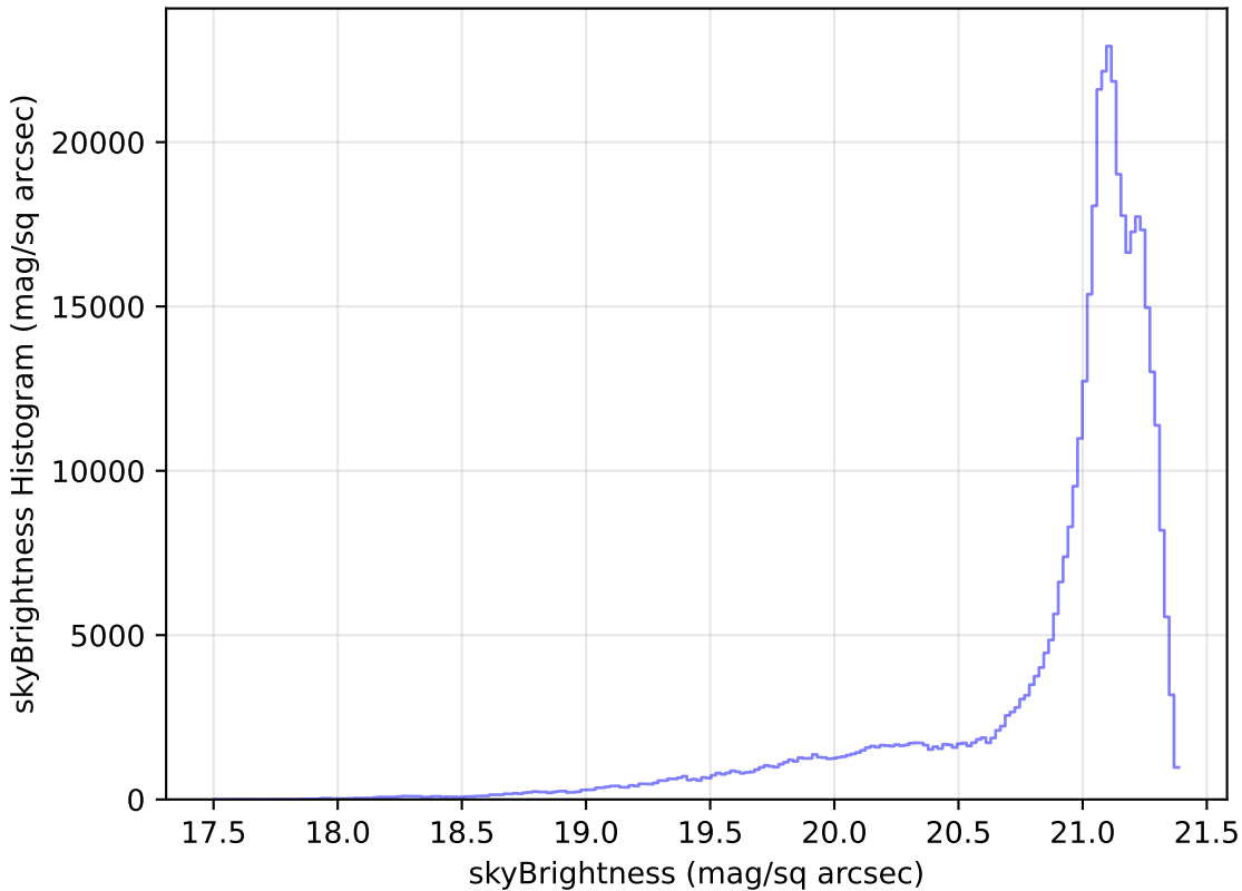
noroll_mjdp120_v3.4_10yrs WFD r band: skyBrightness Histogram
