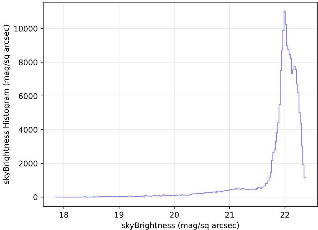
noroll_mjdp120_v3.4_10yrs WFD g band: skyBrightness Histogram
