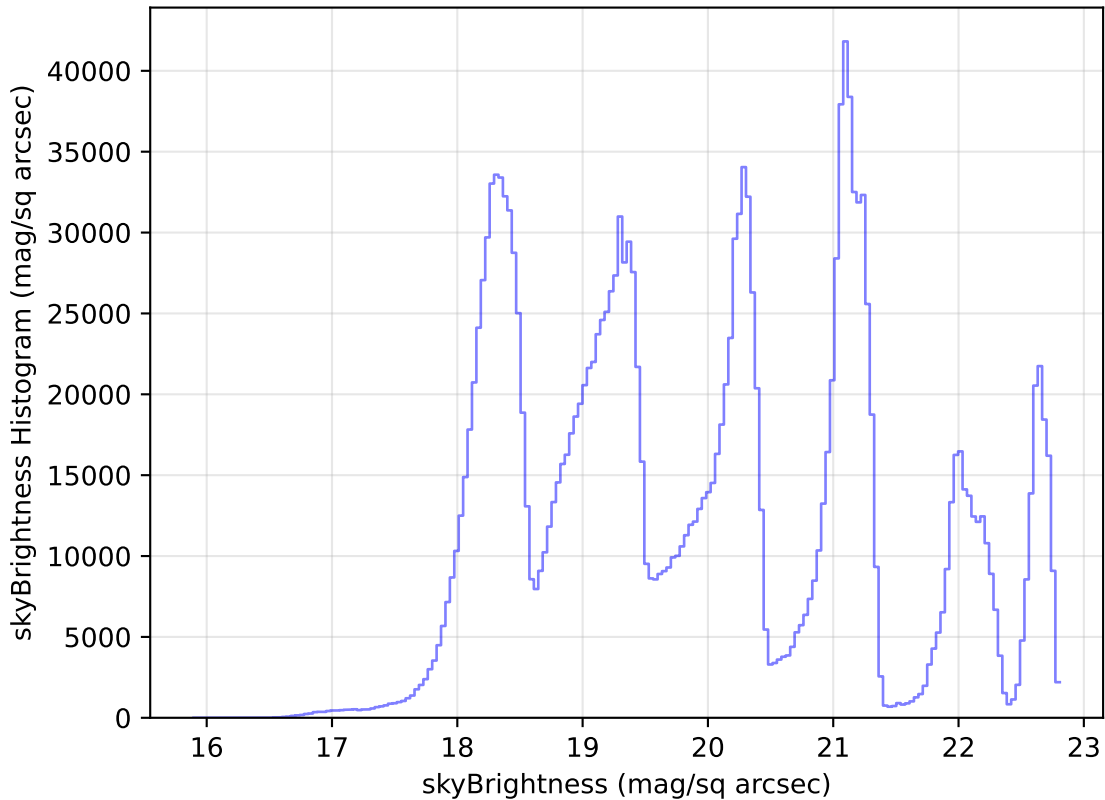
noroll_mjdp120_v3.4_10yrs WFD all bands: skyBrightness Histogram
