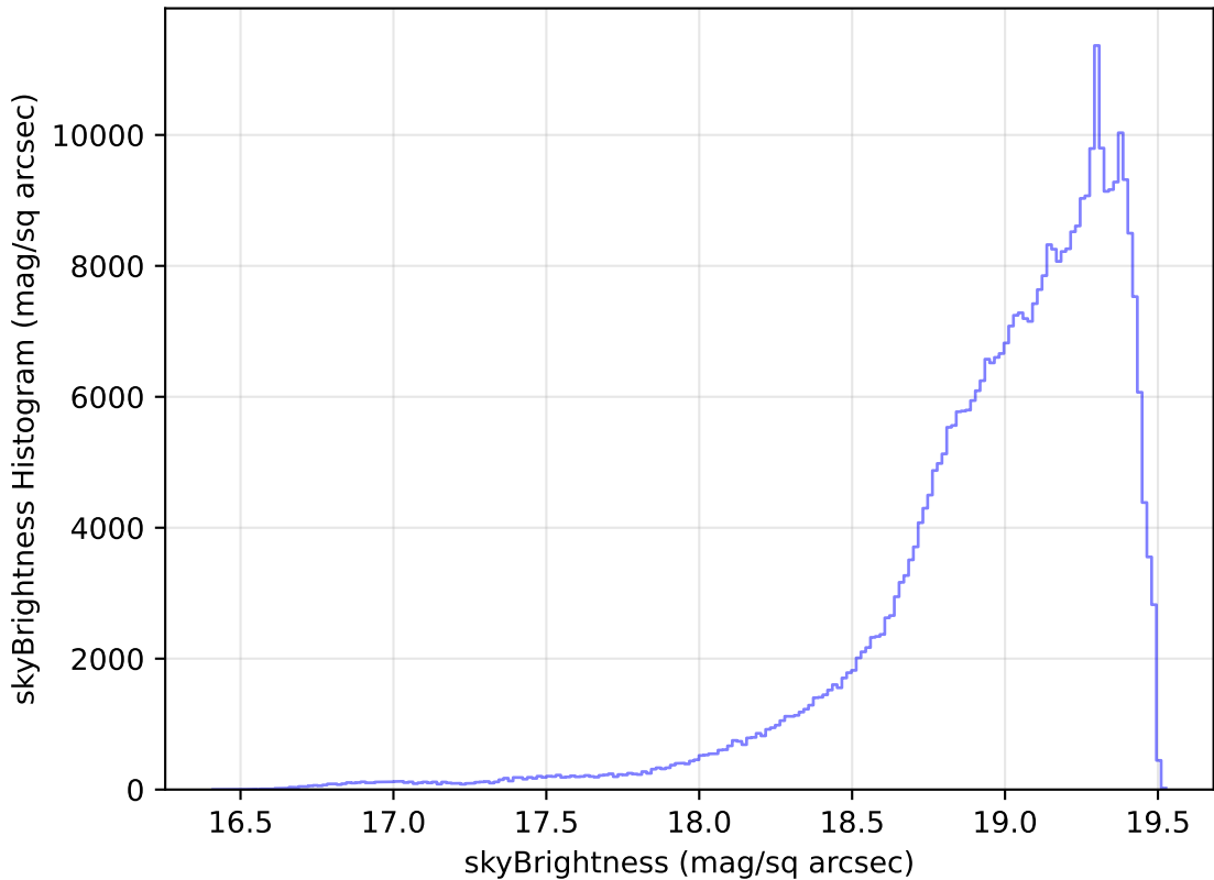
noroll_mjdp120_v3.4_10yrs All sky z band: skyBrightness Histogram
