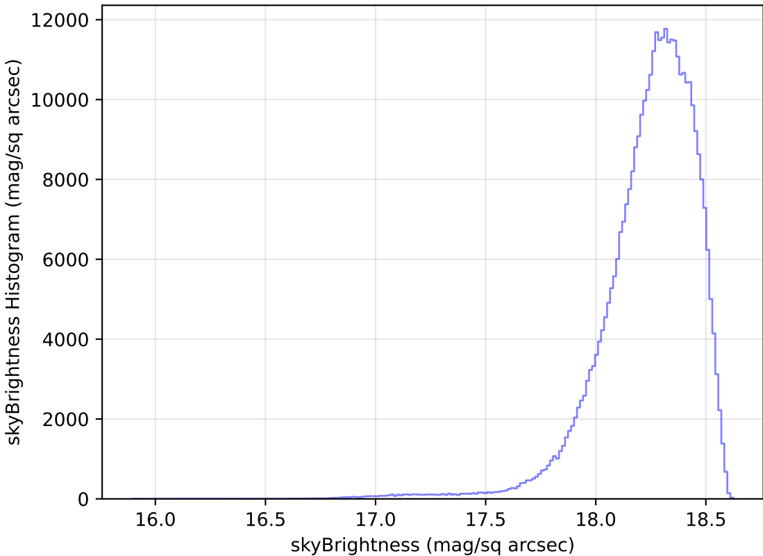
noroll_mjdp120_v3.4_10yrs All sky y band: skyBrightness Histogram
