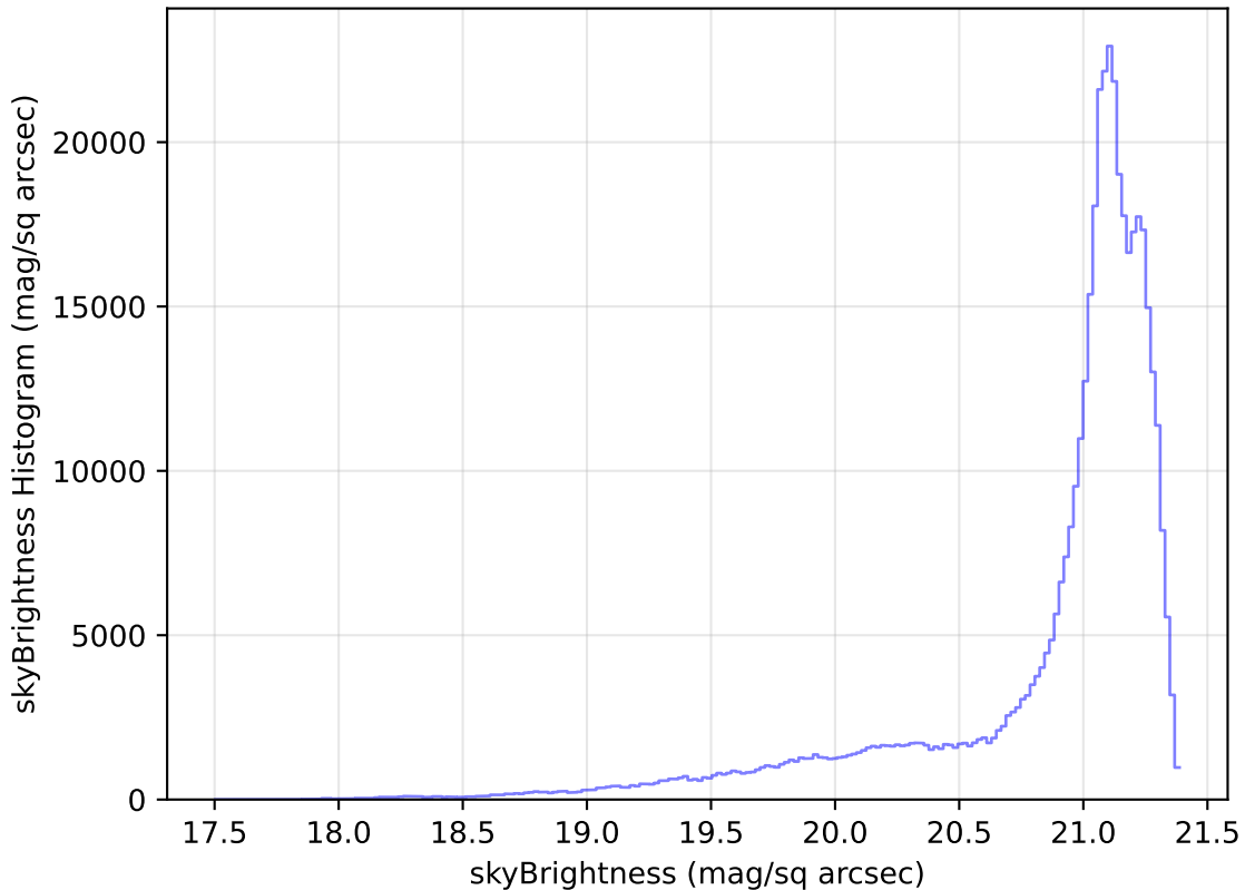
noroll_mjdp120_v3.4_10yrs All sky r band: skyBrightness Histogram
