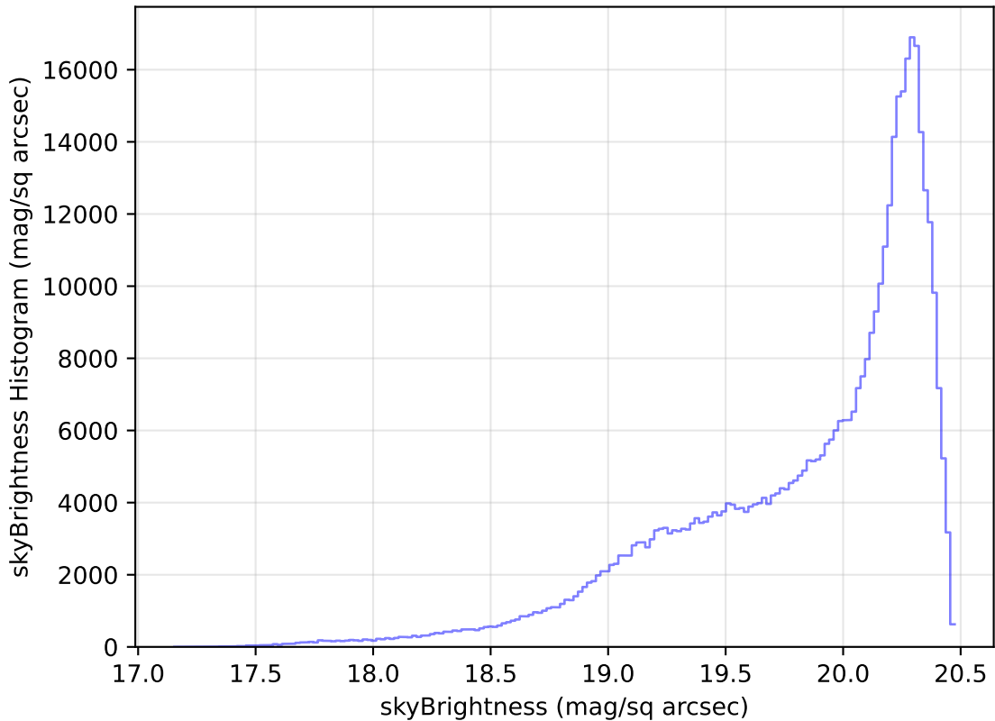
noroll_mjdp120_v3.4_10yrs All sky i band: skyBrightness Histogram
