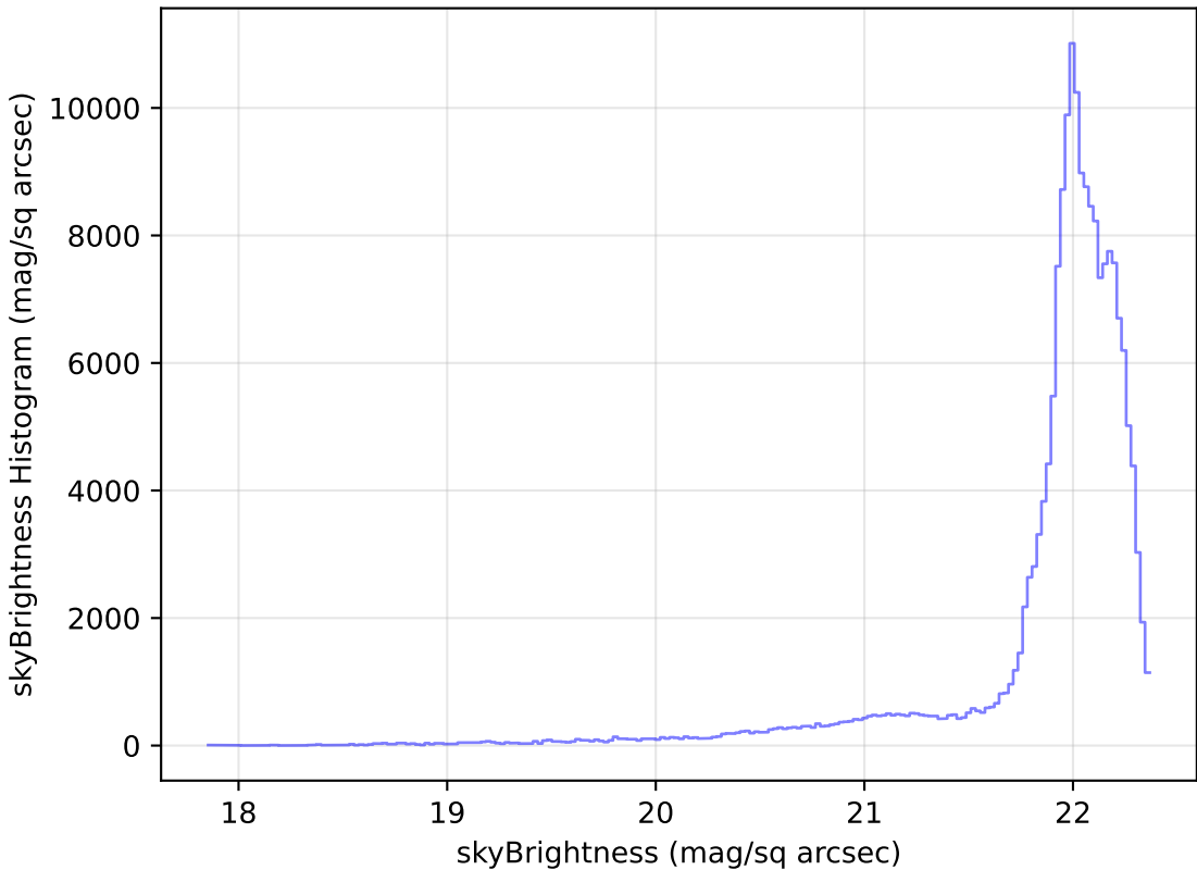
noroll_mjdp120_v3.4_10yrs All sky g band: skyBrightness Histogram
