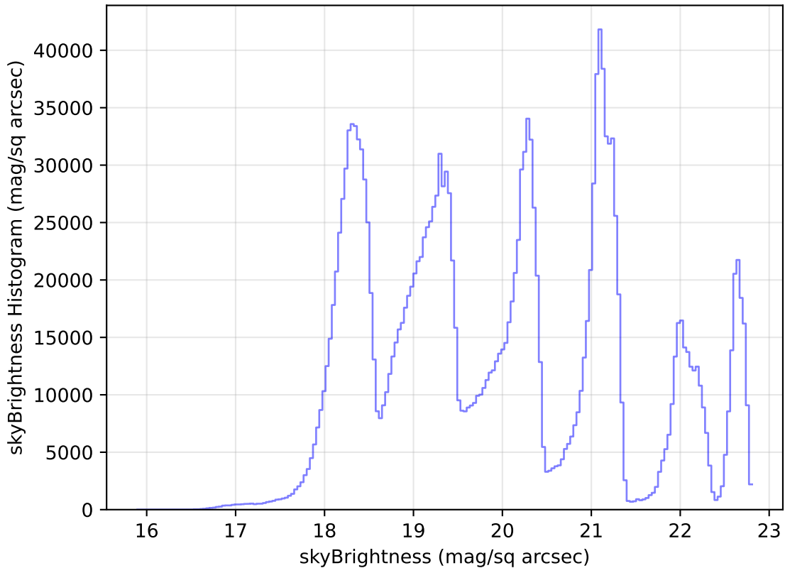
noroll_mjdp120_v3.4_10yrs All sky all bands: skyBrightness Histogram
