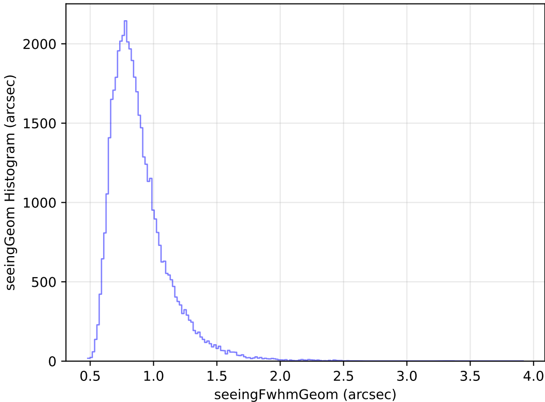
noroll_mjdp120_v3.4_10yrs Yr 1 y band: seeingGeom Histogram
