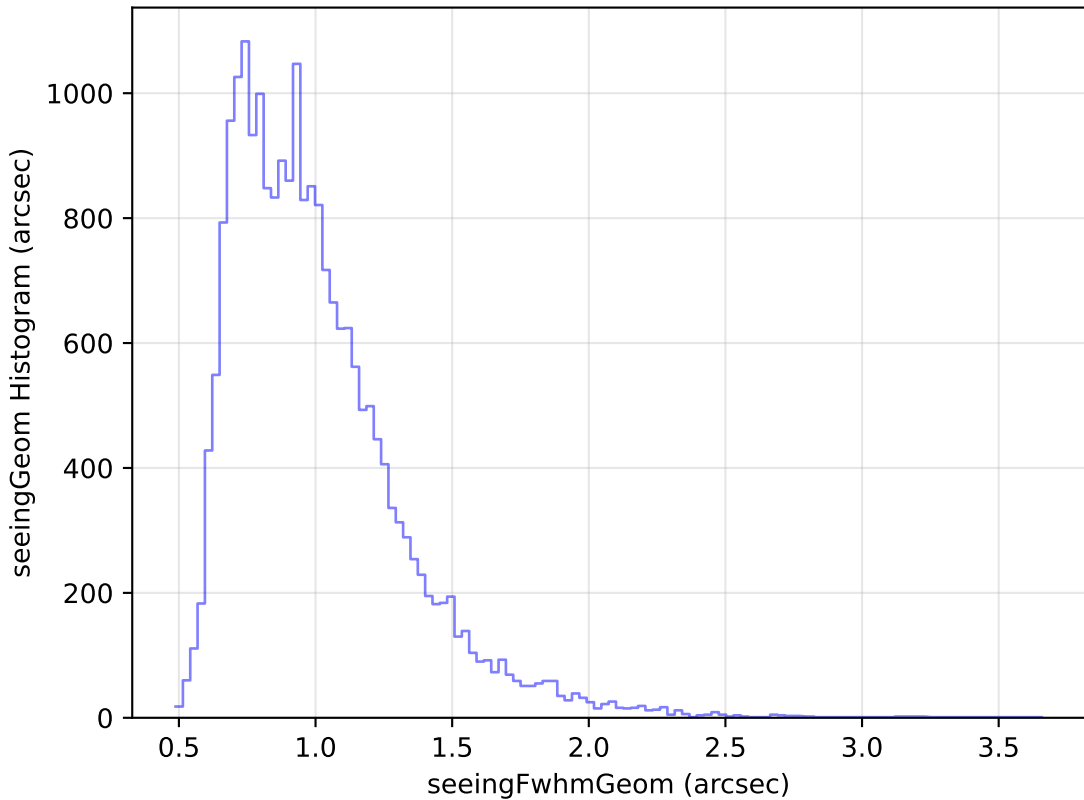
noroll_mjdp120_v3.4_10yrs Yr 1 g band: seeingGeom Histogram
