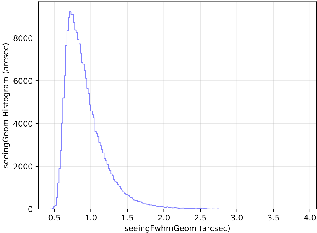
noroll_mjdp120_v3.4_10yrs Yr 1 all bands: seeingGeom Histogram
