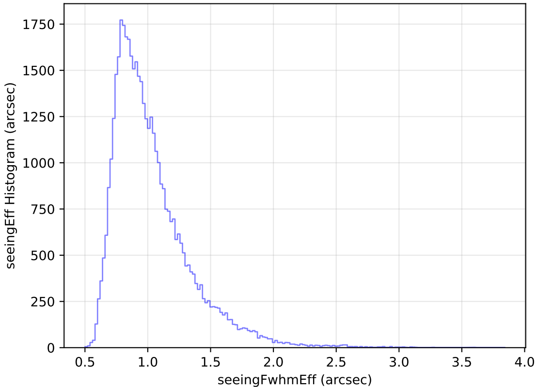
noroll_mjdp120_v3.4_10yrs Yr 1 z band: seeingEff Histogram
