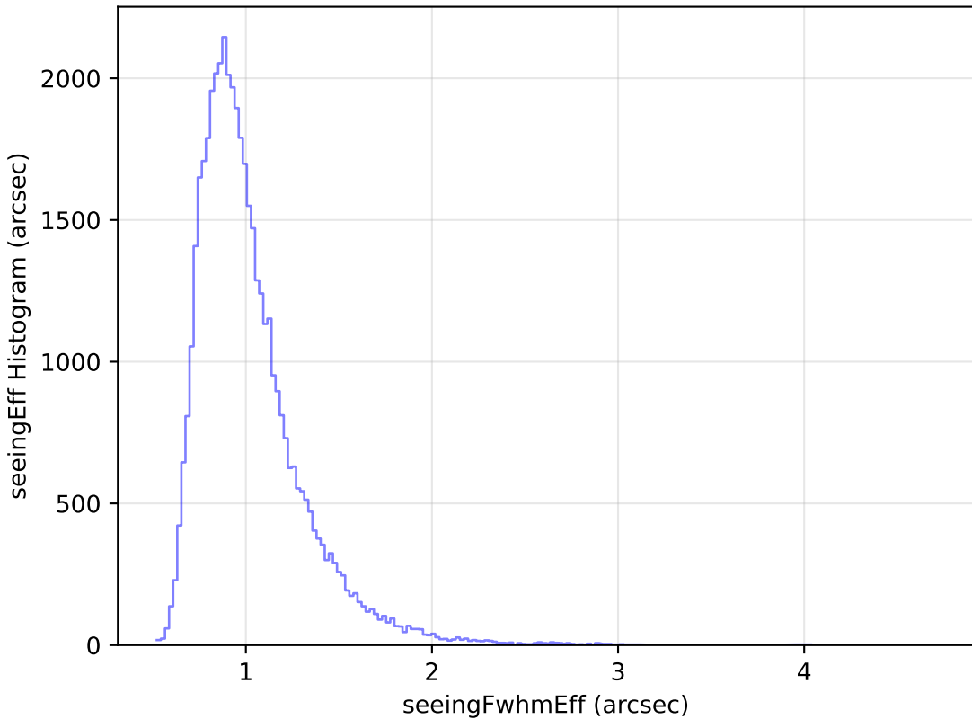
noroll_mjdp120_v3.4_10yrs Yr 1 y band: seeingEff Histogram
