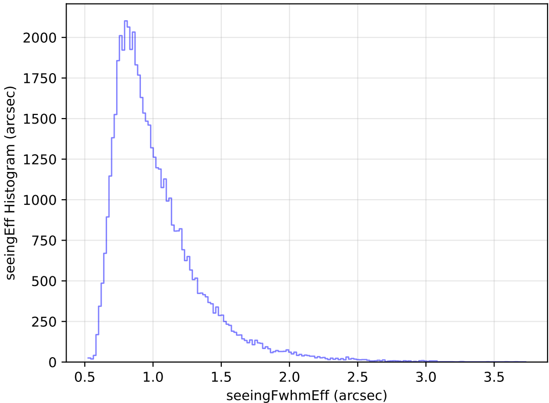
noroll_mjdp120_v3.4_10yrs Yr 1 i band: seeingEff Histogram
