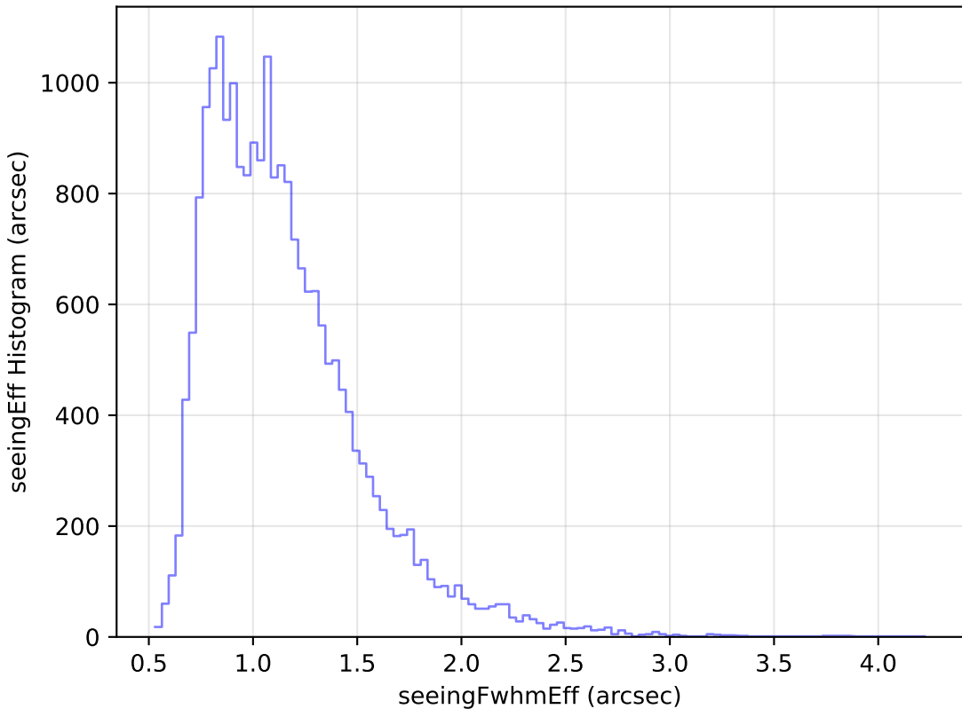
noroll_mjdp120_v3.4_10yrs Yr 1 g band: seeingEff Histogram
