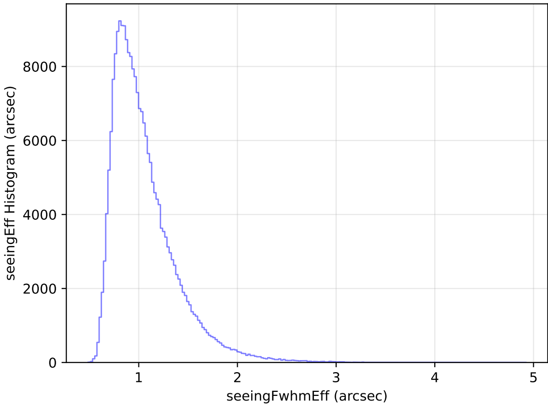
noroll_mjdp120_v3.4_10yrs Yr 1 all bands: seeingEff Histogram
