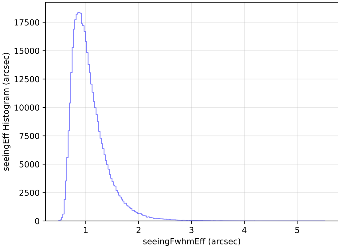
noroll_mjdp120_v3.4_10yrs WFD z band: seeingEff Histogram
