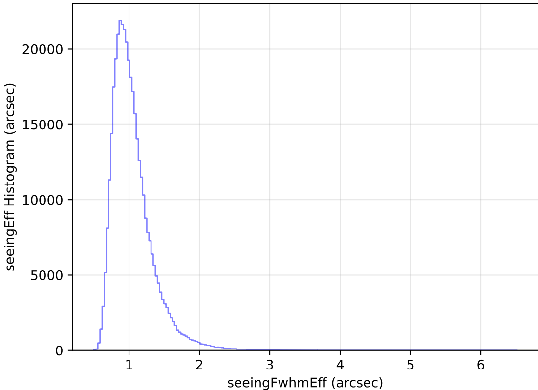
noroll_mjdp120_v3.4_10yrs WFD y band: seeingEff Histogram
