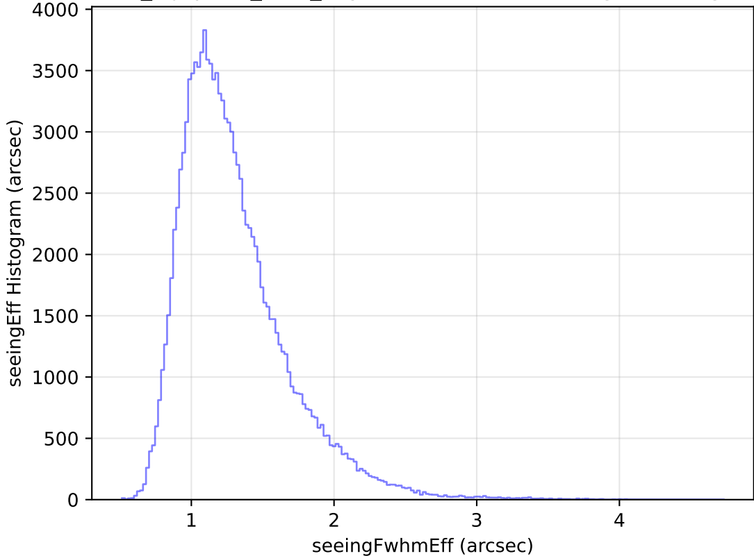
noroll_mjdp120_v3.4_10yrs WFD u band: seeingEff Histogram
