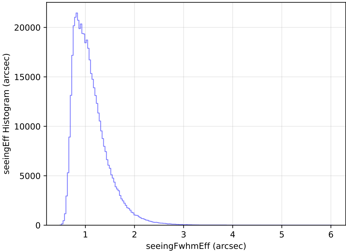
noroll_mjdp120_v3.4_10yrs WFD r band: seeingEff Histogram
