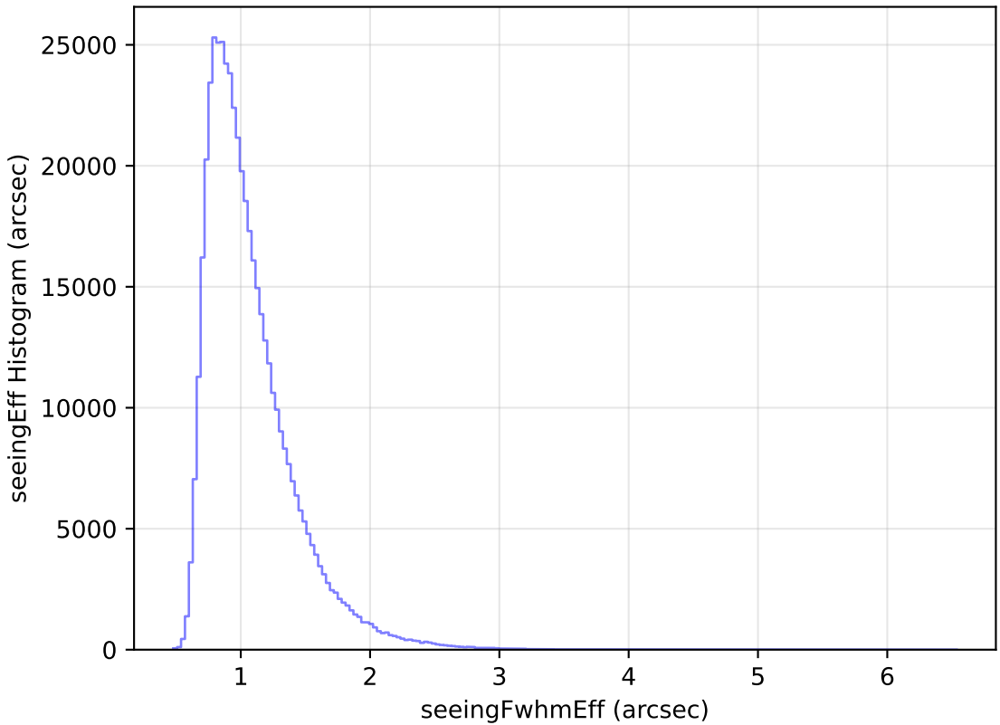
noroll_mjdp120_v3.4_10yrs WFD i band: seeingEff Histogram
