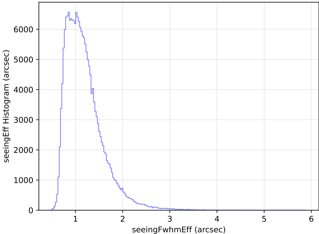
noroll_mjdp120_v3.4_10yrs WFD g band: seeingEff Histogram
