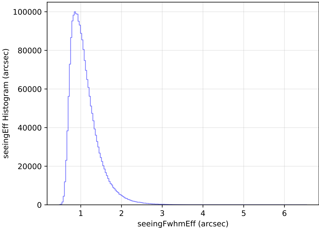
noroll_mjdp120_v3.4_10yrs WFD all bands: seeingEff Histogram
