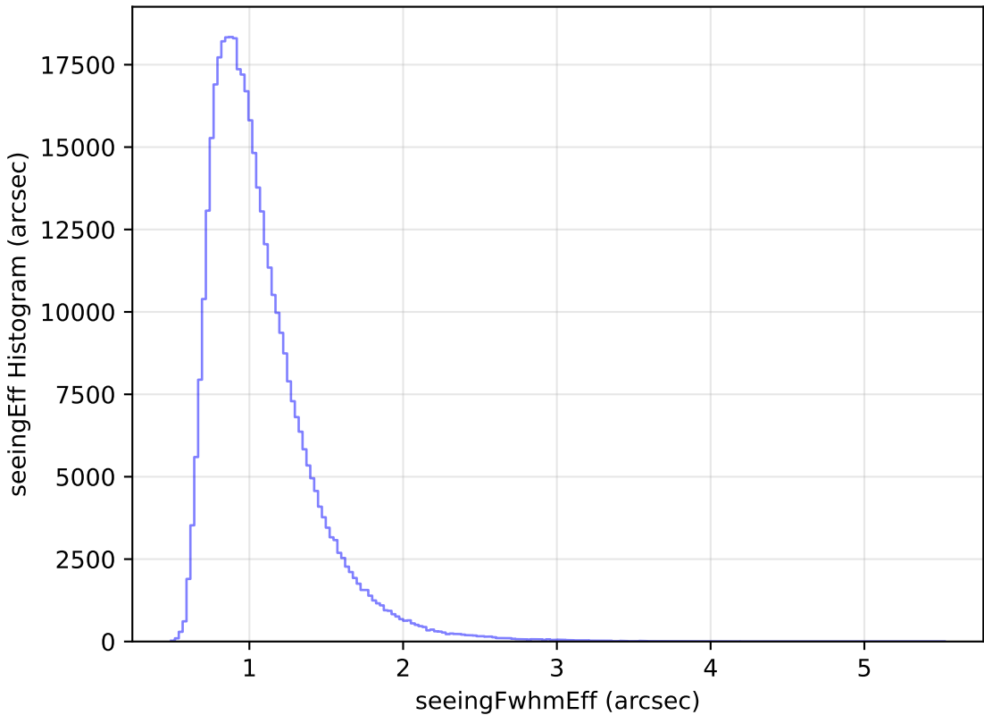
noroll_mjdp120_v3.4_10yrs All sky z band: seeingEff Histogram
