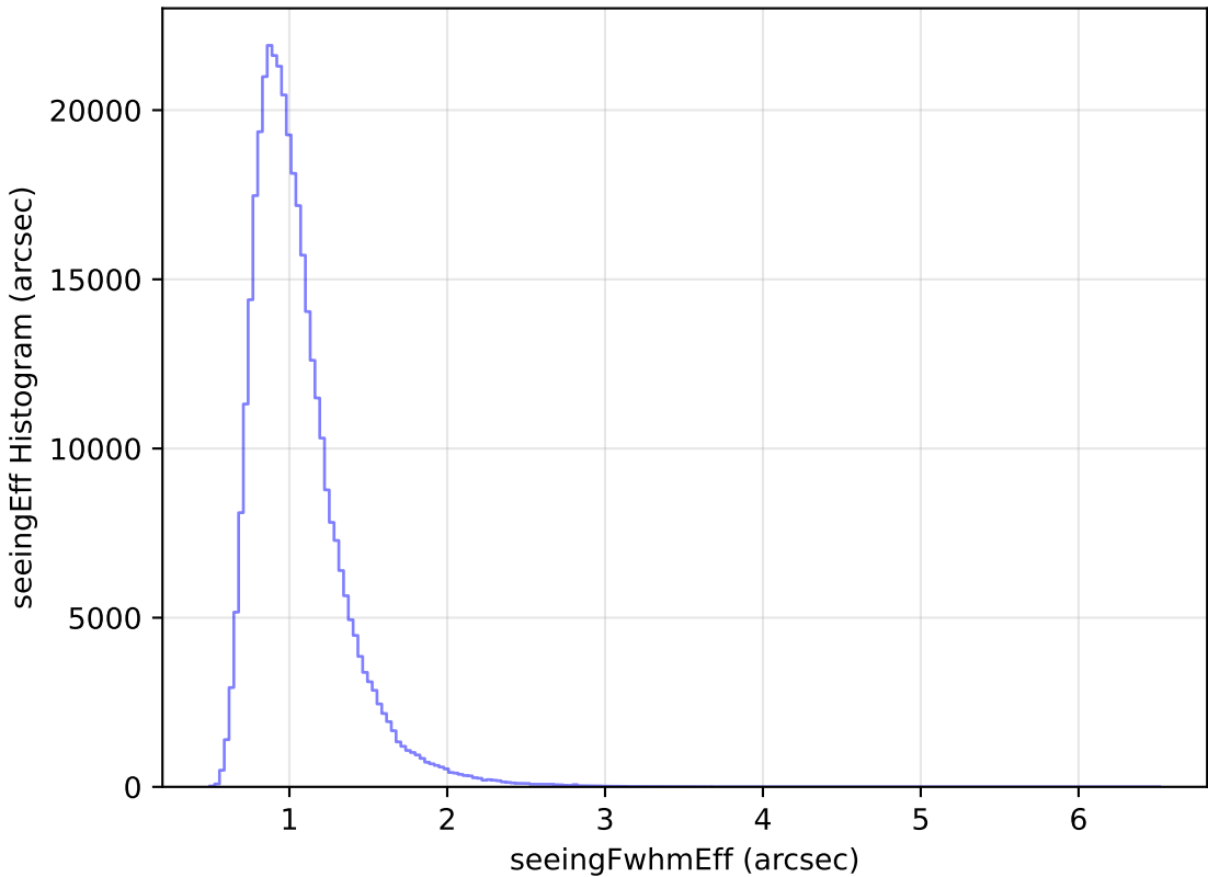
noroll_mjdp120_v3.4_10yrs All sky y band: seeingEff Histogram
