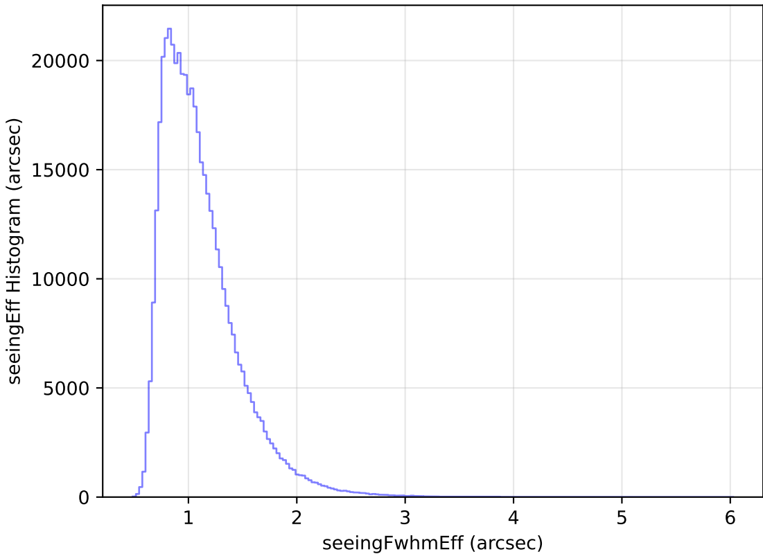
noroll_mjdp120_v3.4_10yrs All sky r band: seeingEff Histogram
