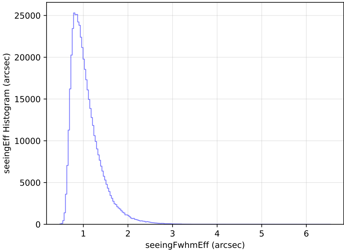
noroll_mjdp120_v3.4_10yrs All sky i band: seeingEff Histogram
