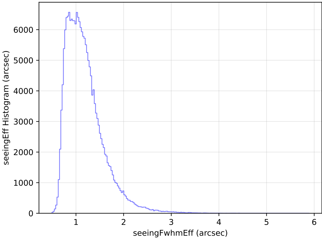
noroll_mjdp120_v3.4_10yrs All sky g band: seeingEff Histogram
