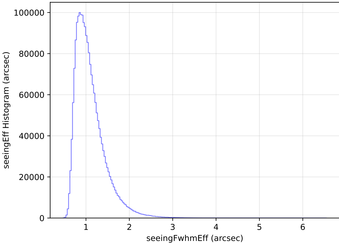
noroll_mjdp120_v3.4_10yrs All sky all bands: seeingEff Histogram
