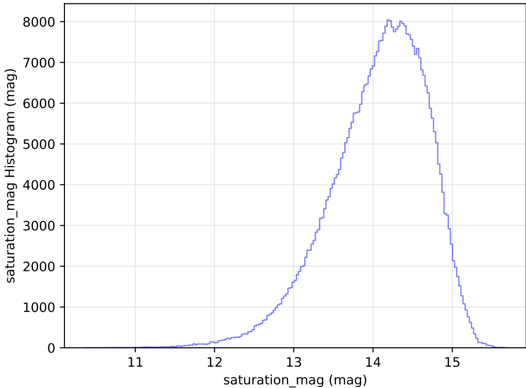
noroll_mjdp120_v3.4_10yrs WFD z band: saturation_mag Histogram
