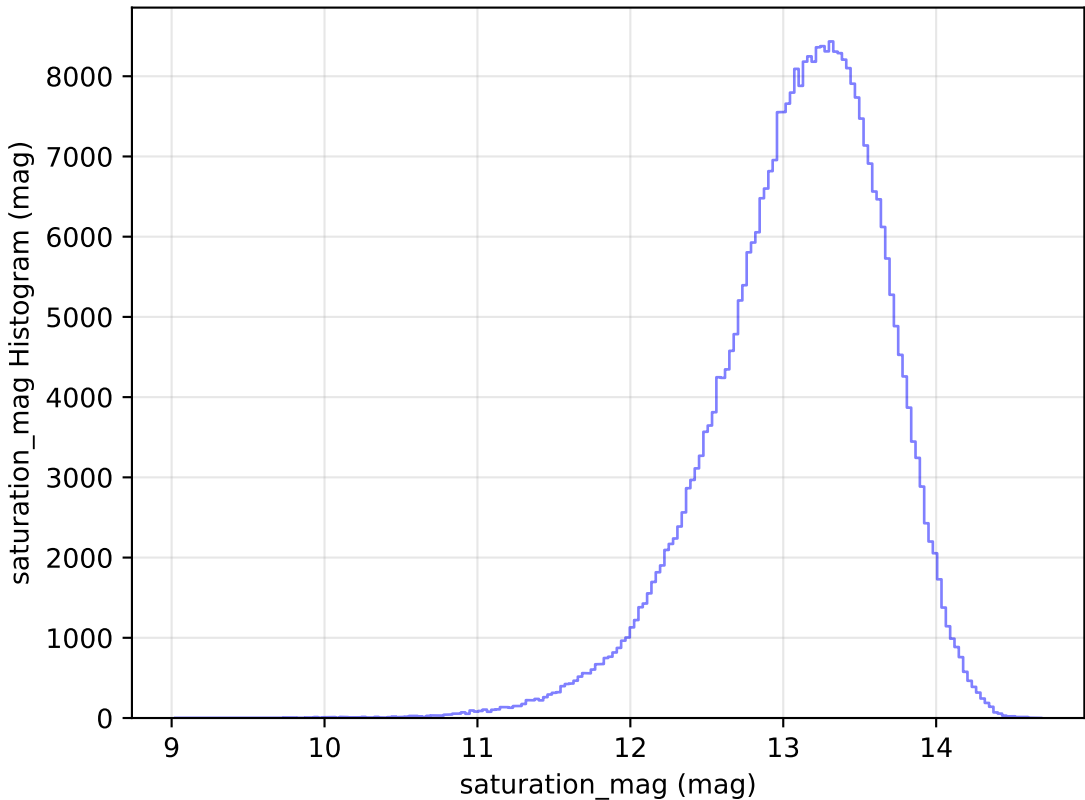
noroll_mjdp120_v3.4_10yrs WFD y band: saturation_mag Histogram
