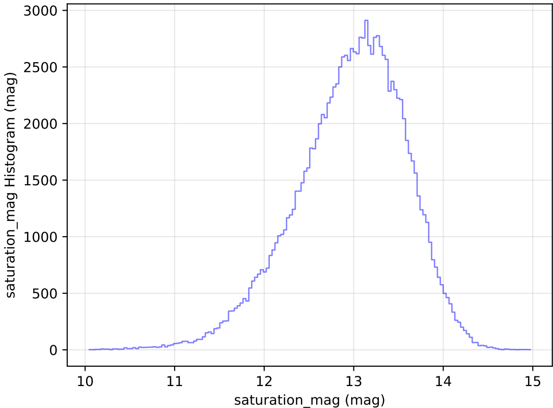
noroll_mjdp120_v3.4_10yrs WFD u band: saturation_mag Histogram
