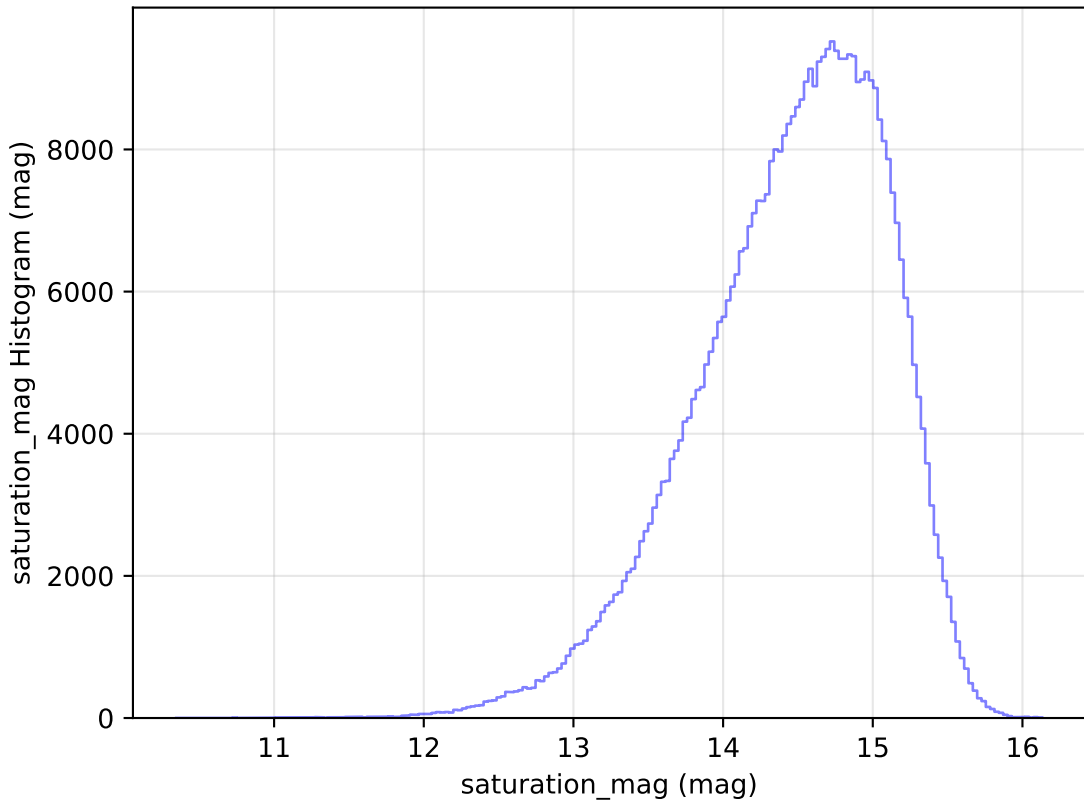
noroll_mjdp120_v3.4_10yrs WFD i band: saturation_mag Histogram
