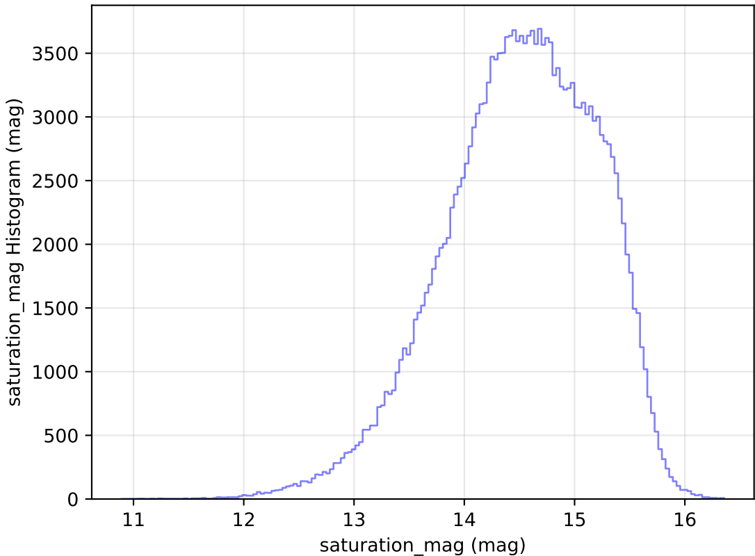
noroll_mjdp120_v3.4_10yrs WFD g band: saturation_mag Histogram
