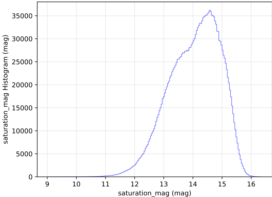
noroll_mjdp120_v3.4_10yrs WFD all bands: saturation_mag Histogram
