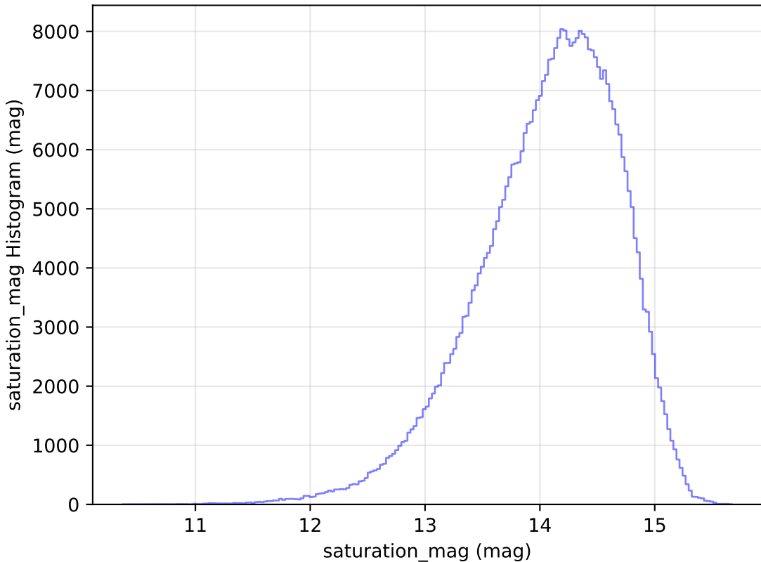
noroll_mjdp120_v3.4_10yrs All sky z band: saturation_mag Histogram
