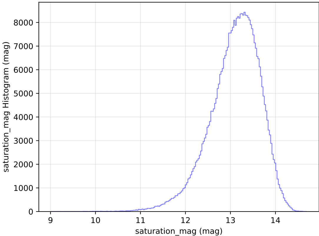
noroll_mjdp120_v3.4_10yrs All sky y band: saturation_mag Histogram
