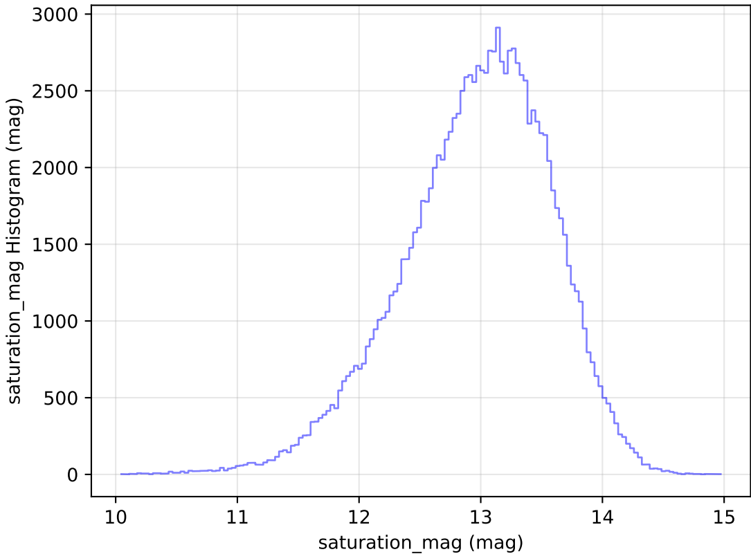
noroll_mjdp120_v3.4_10yrs All sky u band: saturation_mag Histogram
